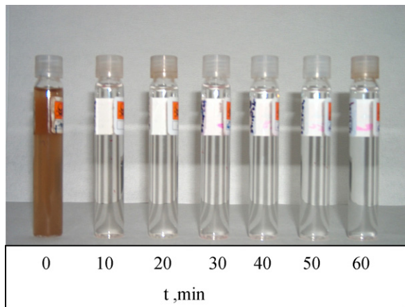
Fig. 10. Color change in the effluent with electrolysis time. pH: 7.8, j : 20 mA cm -2 , C_{Na_2SO_4} : 0.05 M, 0.75 g L -1 PAC. (For interpretation of the references to color in this figure legend, the reader is referred to the web version of the article.)
