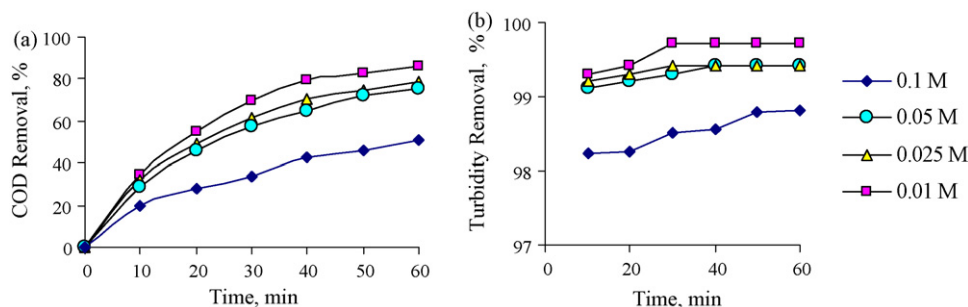
Fig. 7. Effect of salt concentration on COD removal (a) and turbidity removal (b) at aluminum electrode. pH: 7.8, j : 20 mA cm -2 .
