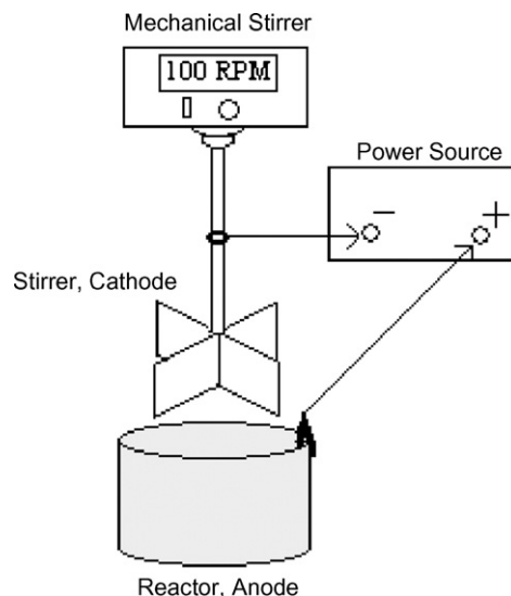
Fig. 1. Experimental setup.
