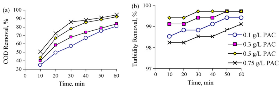
Fig. 9. Effect of PAC concentration on COD removal (a) and turbidity removal (b) at aluminum electrodes. pH: 7.8, j : 20 mA cm -2 , C_{Na_2SO_4} : 0.05 M.
