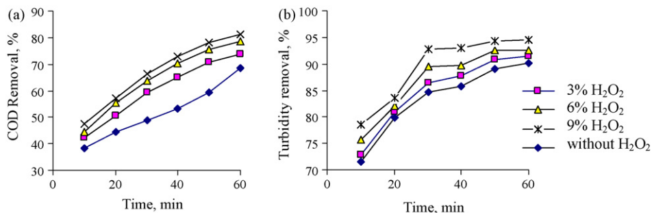
Fig. 11. Effect of H 2 O 2 concentration on COD removal (a) and turbidity removal (b) at iron electrodes. pH: 7.8, j : 20 mA cm -2 .
