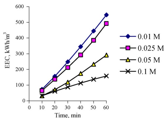
Fig. 8. Effect of salt concentration on EEC for aluminum electrode. pH: 7.8, j : 20 mA cm -2 .
